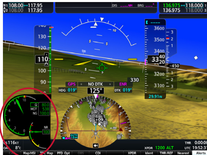
Power Situation Indicator.
