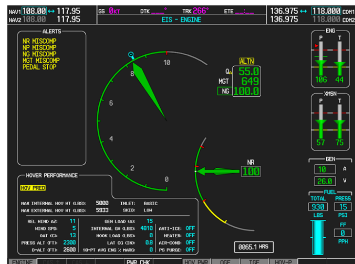
Pre-flight planning hover performance check (HOV-Predictive Mode).
